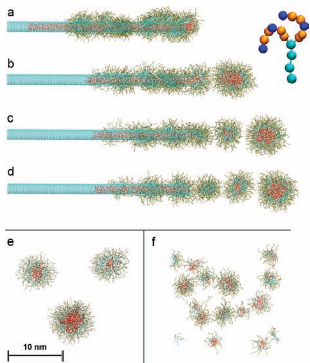
Figure 1. Controlled self-assembly of hydrated double-headed lipid micelles filled with hexadecane. (a) Lipids deposited on the CNT form random hemimicelles after 20 ns. (b–d) Micelles with kinetically controlled sizes and filling are sequentially formed at the CNT tip when the hexadecane molecules in the CNT interior are pressurized and the lipids on its surface are dragged by the water flowing around it. The inset shows a single biheaded lipid molecule. Color scheme: red, CG hexadecane; gray, hydrophilic lipid head; cyan, hydrophobic lipid tail. See the movie in the Supporting Information. (e) Three hexadecane-filled micelles from (d) after 400 ns of equilibration. (f) Thermodynamically driven self-assembly of double-headed lipid monomers and hexadecane in water for the same system as in (d). After 300 ns of equilibration, the sizes of the micelles and their filling are largely random.
