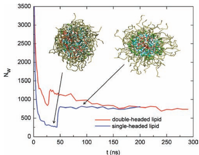
Figure 3. Number of water molecules present within 0.5 nm (first monolayer) of the hydrophobic micelle core during the self-assembly of hydrated double-headed (red) and single-headed (blue) lipid monomers into micelles filled with hexadecane. The inset shows different forms of one micelle selected from the system of self-assembling single-headed lipid monomers.
