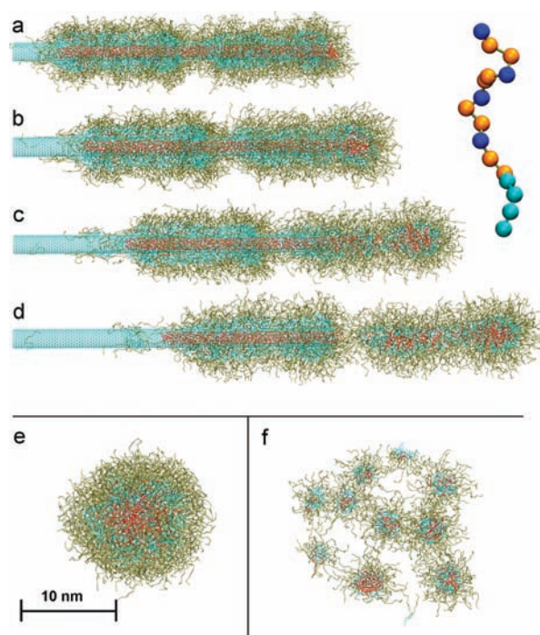
Figure 2. Controlled self-assembly of hydrated single-headed lipid bicelles filled with hexadecane. (a) Lipids deposited on the CNT form random tubular structures after 20 ns. (b–d) Bicelles with kinetically controlled sizes and filling are sequentially formed at the CNT tip when the hexadecane molecules in the CNT interior are pressurized and the lipids on its surface are dragged by the water flowing around it. The inset shows single single-headed lipid molecule. Color scheme: red, CG hexadecane; gray, hydrophilic lipid head; cyan, hydrophobic lipid tail. See the movie in the Supporting Information. (e) Hexadecane-filled bicelle from (d) after 375 ns of equilibration. (f) Thermodynamically driven self-assembly of single-headed lipid monomers and hexadecane in water for the same system as in (d). After 450 ns of equilibration, the sizes of the micelles and their filling are largely random.
